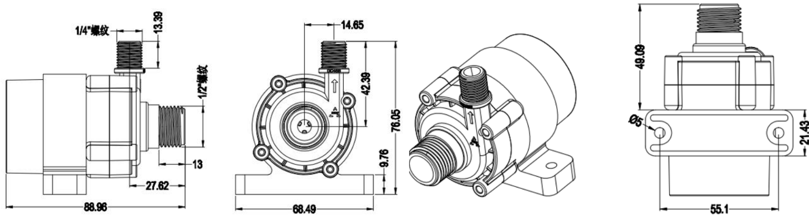
DC45I 泵头 Pump Head DC45I
