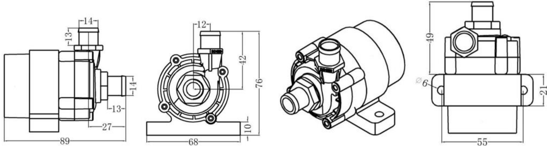
DC45D 泵头 Pump Head DC45D
