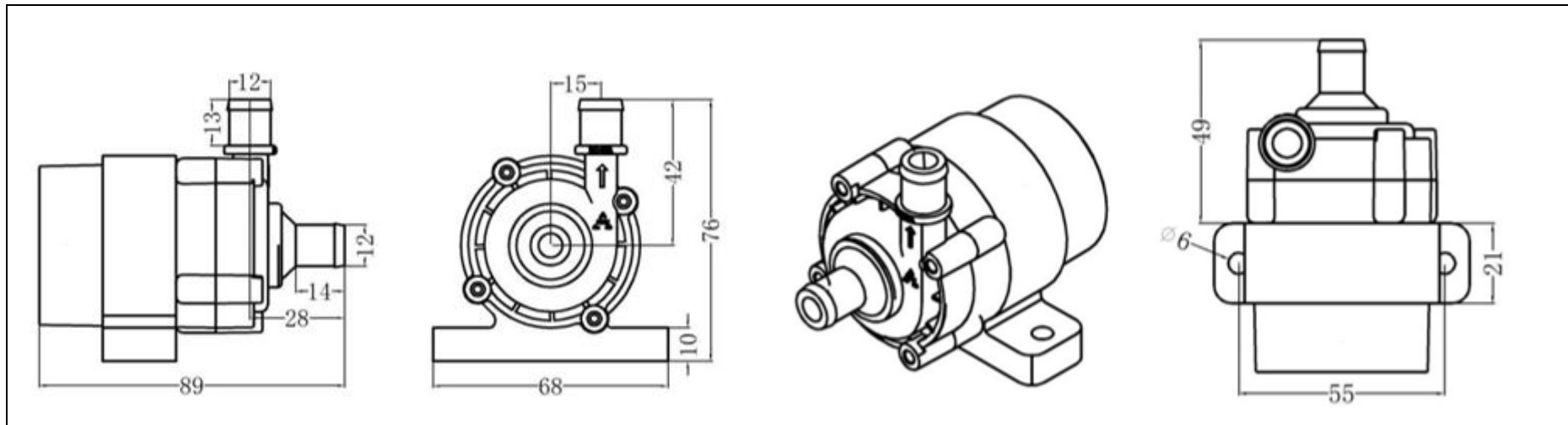
DC45B 泵头 Pump Head DC45B
