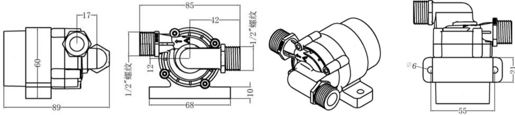
DC45D 泵头 Pump Head DC45D
