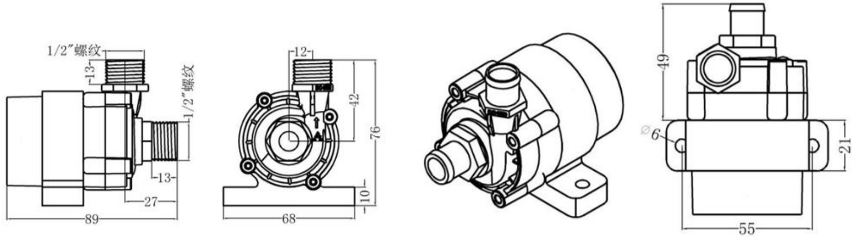
DC45I 泵头 Pump Head DC45I
