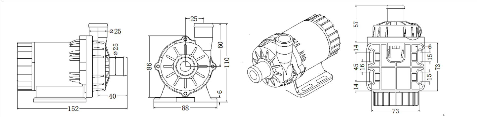
DC60D 泵头 Pump Head DC60D
