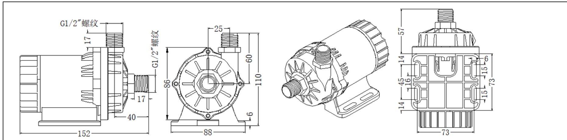
DC60G 泵头 Pump Head DC60G
