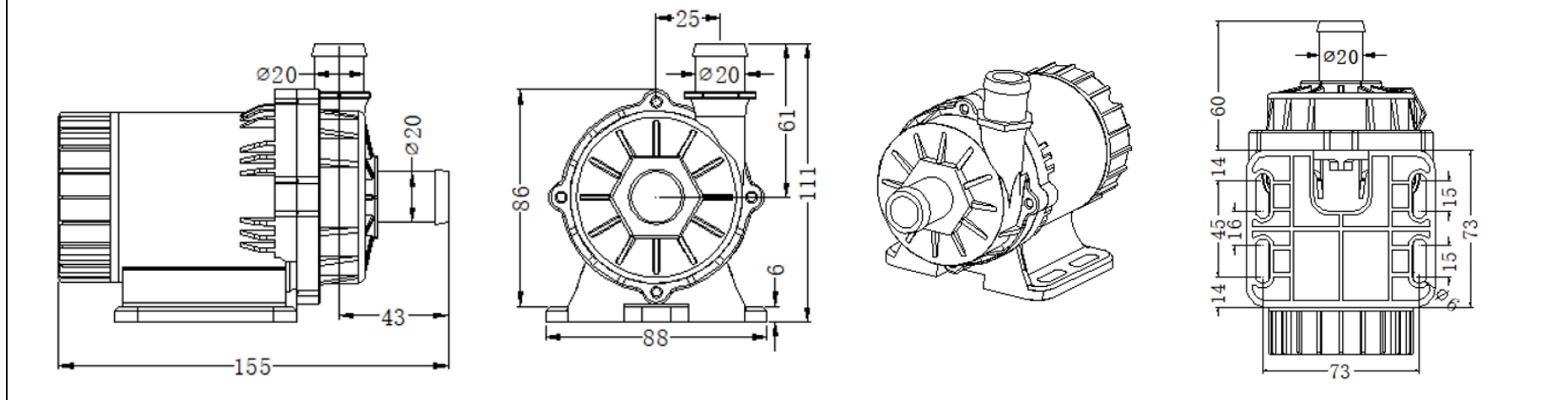
DC60E 泵头 Pump Head DC60E
