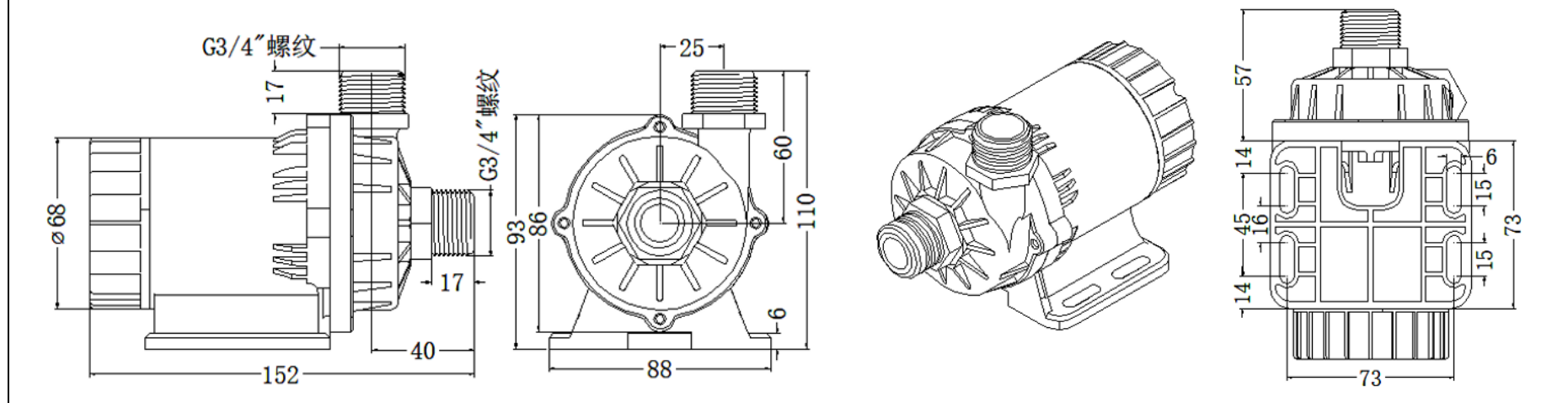
水泵驱动内外置版本图解 Diagram of internal and external versions of water pump driven.
